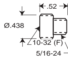
PMCM-* Straight-thru Socket
