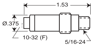
PMCIL-* Valved Inline Socket
