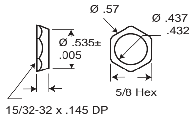
15/32-32 x .145 DP DP-22 DP-11
